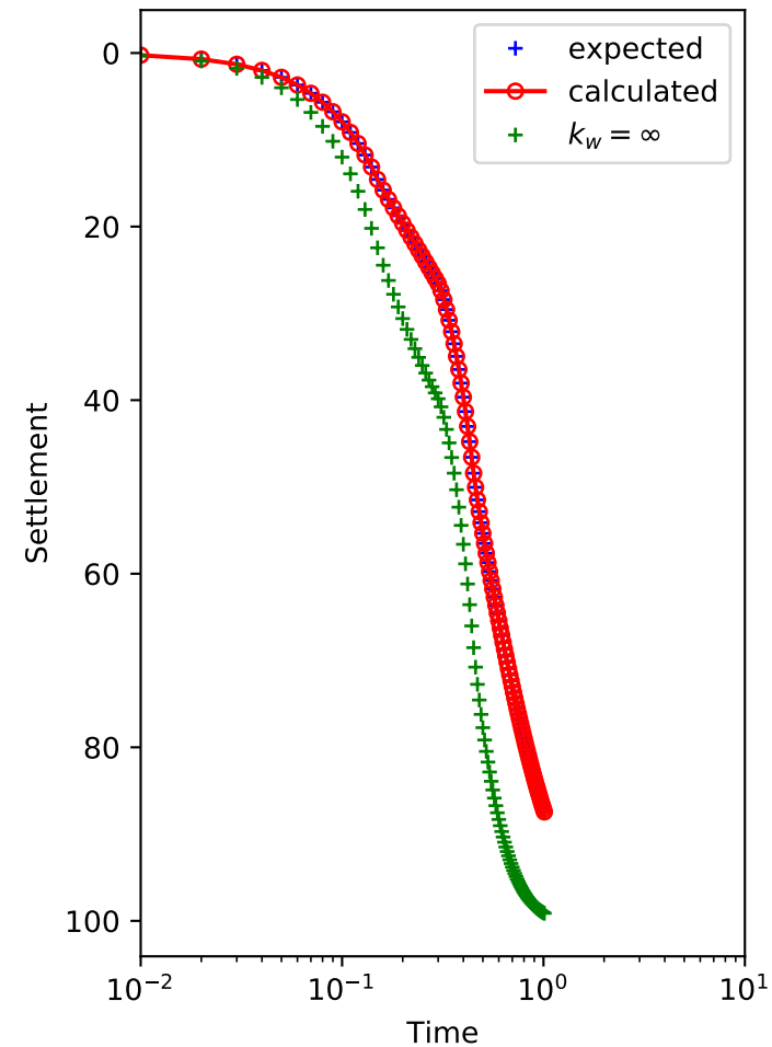
Tang and Onitsuka (2000) vertical and radial drainage including well resistance
