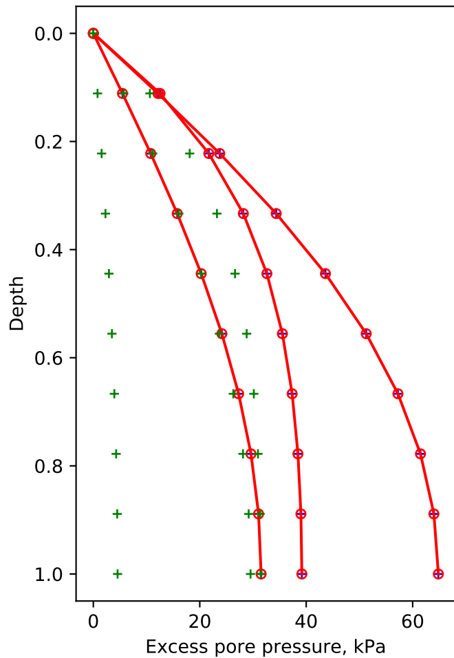
Tang and Onitsuka (2000) vertical and radial drainage including well resistance
