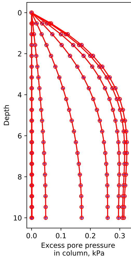
Lu et al (2010) Stone column, load is linear with depth
