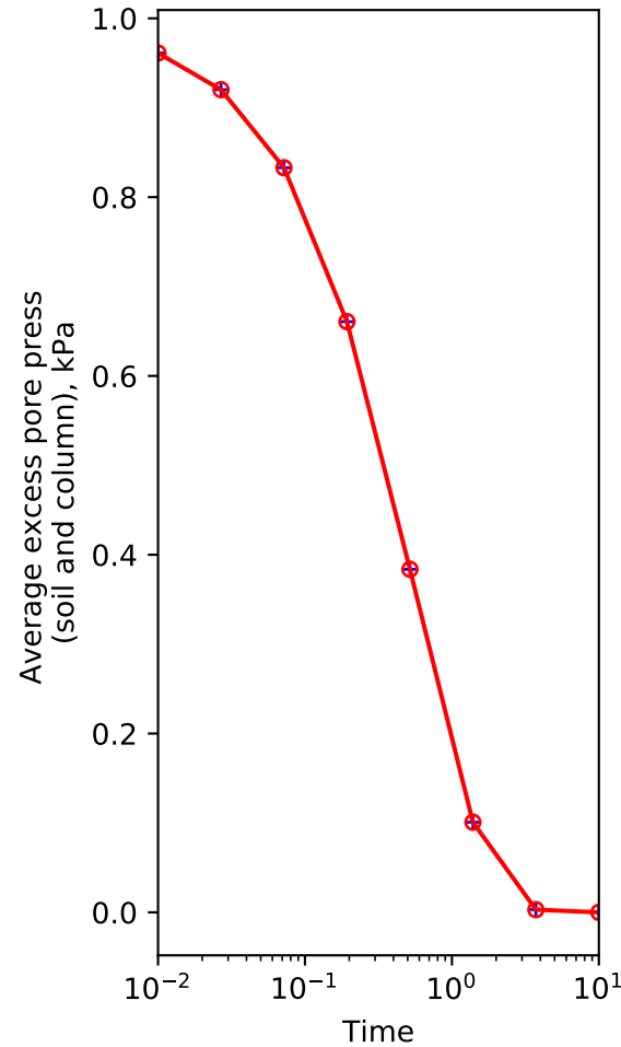
Lu et al (2010) Stone column, load is uniform with depth
