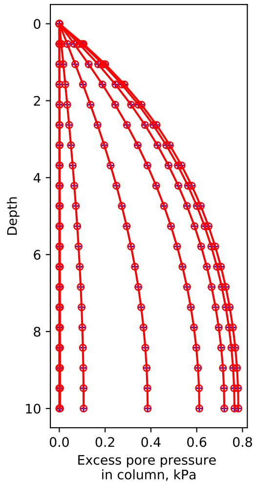
Lu et al (2010) Stone column, load is uniform with depth
