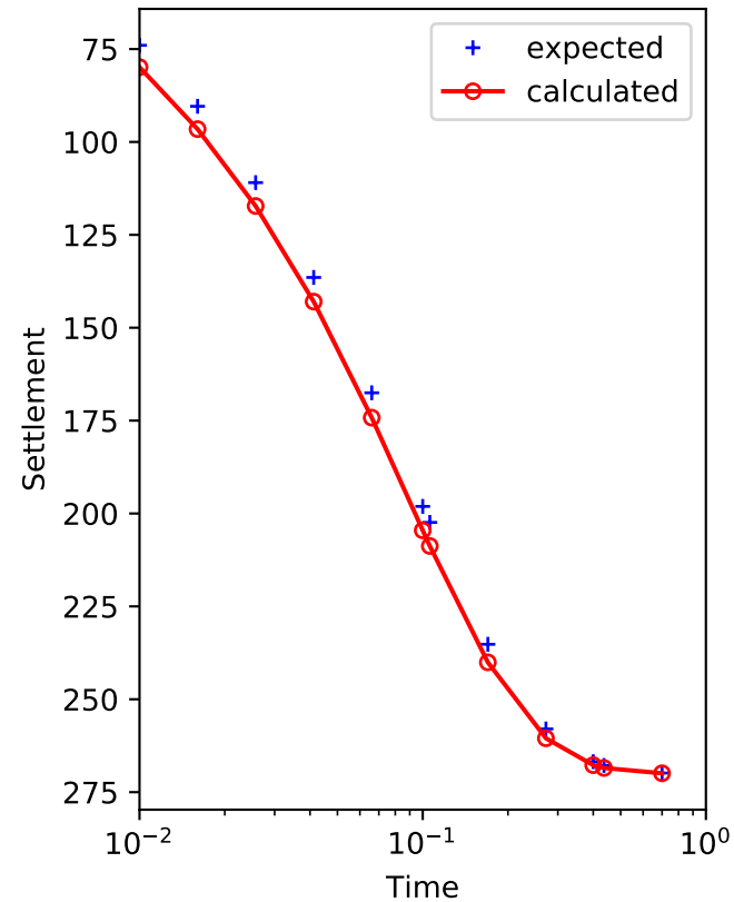
Nogami and li (2003) vertical and radial drainage free strain vs equal strain. Lambda=100
