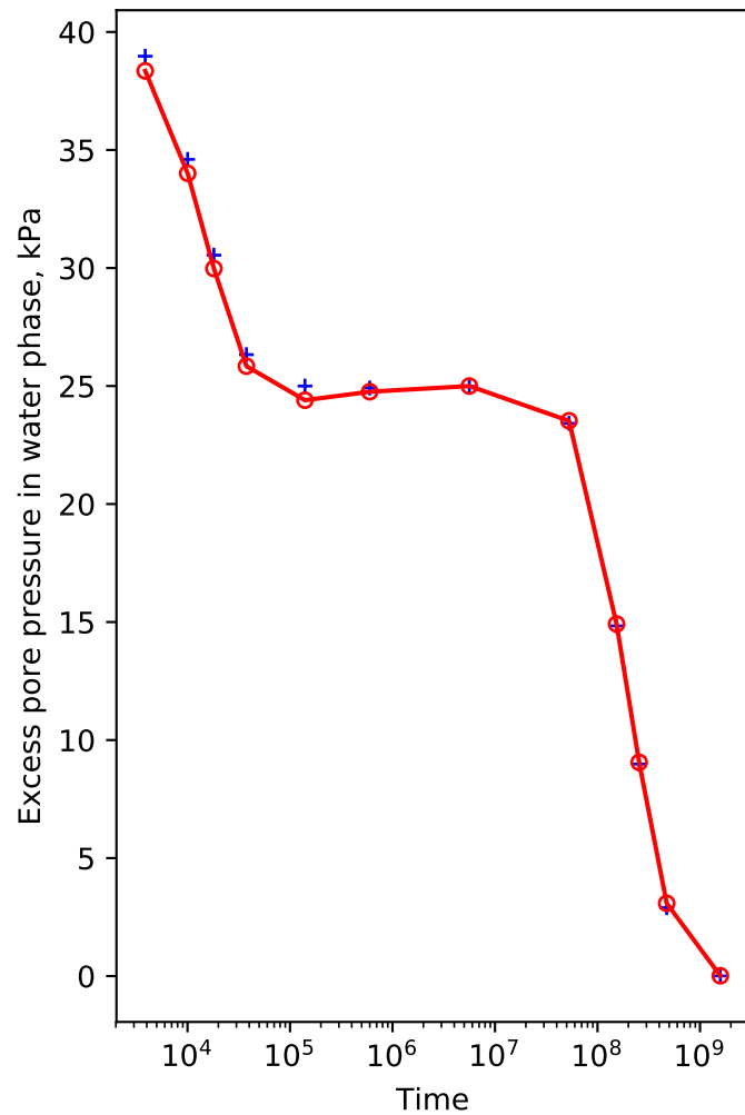
Shan et al. (2012) Unsaturated soil, instant surcharge, k_a/k_w=100 Fig2a and Fig5a
