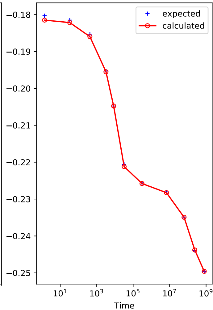
Shan et al. (2012) Unsaturated soil, instant surcharge, k_a/k_w=100 Fig2a and Fig5a
