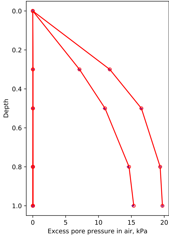
Shan et al. (2012) Unsaturated soil. instant surcharge + sinusoidal top water pressure boundary condition.
